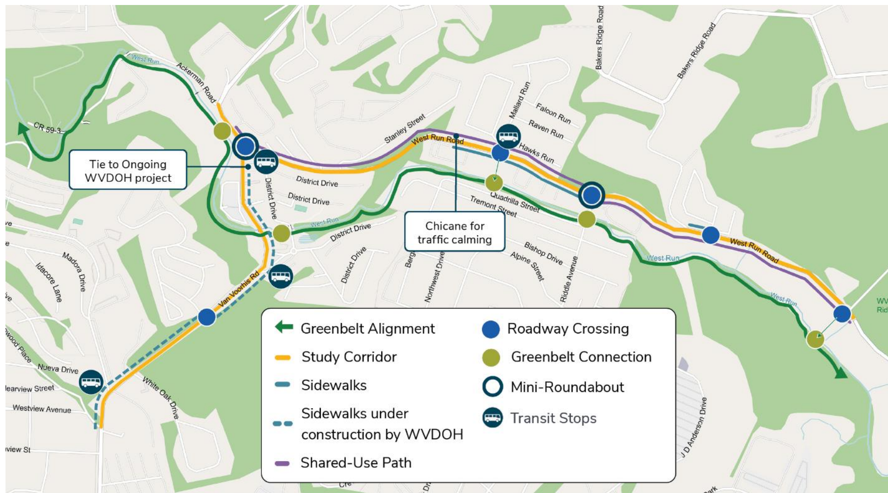
Figure 38: Preferred Concept
